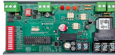
Code Version 1.5
