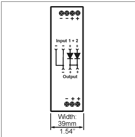
Fig. 16-1 Front view
