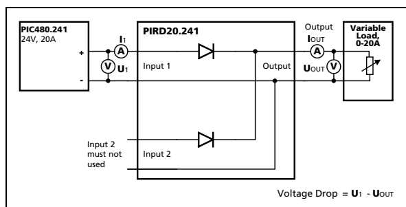
Fig. 17-2 Test setup for voltage drop measurements
