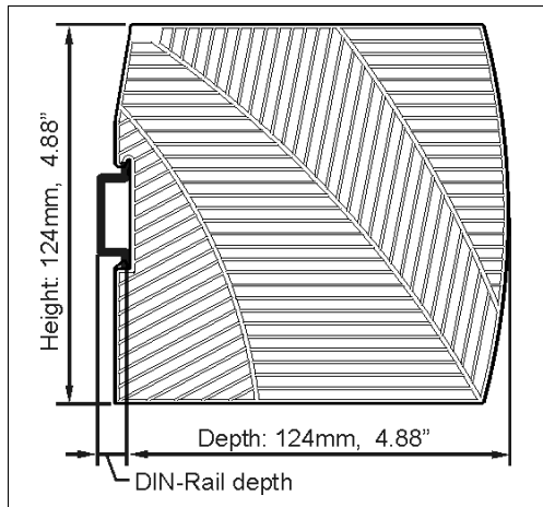
Fig. 16-2 Side view
