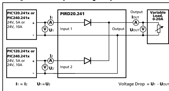
Fig. 3-2 Test setup for voltage drop measurements
