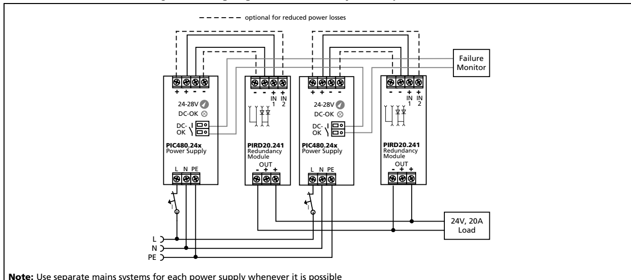
Fig. 17-4 Wiring diagram, 1+1 Redundancy, 20A output current
