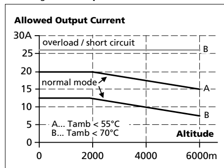
Fig. 10-2 Output current vs. altitude
