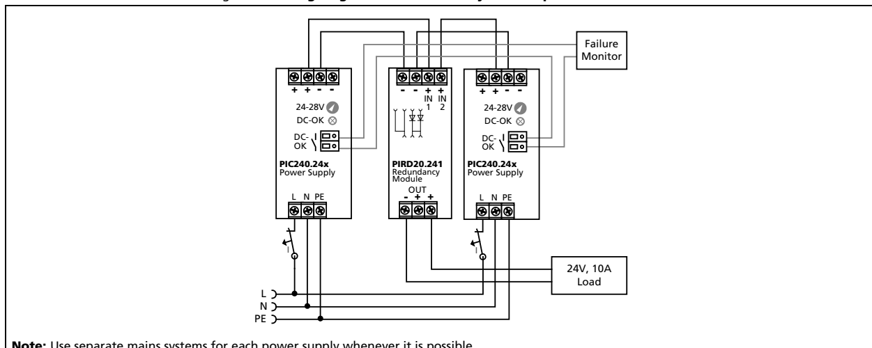
Fig. 17-3 Wiring diagram, 1+1 Redundancy, 10A output current
