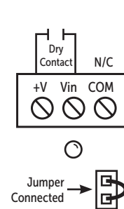
Example of Dry Contact Input Operation
