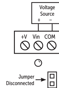
Example of Voltage Input Operation
